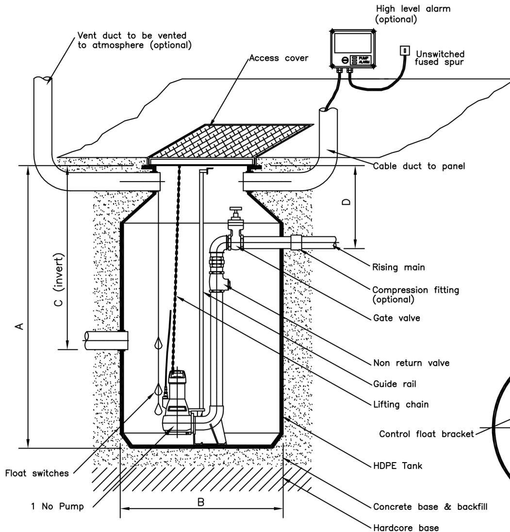
SIDE ELEVATION
