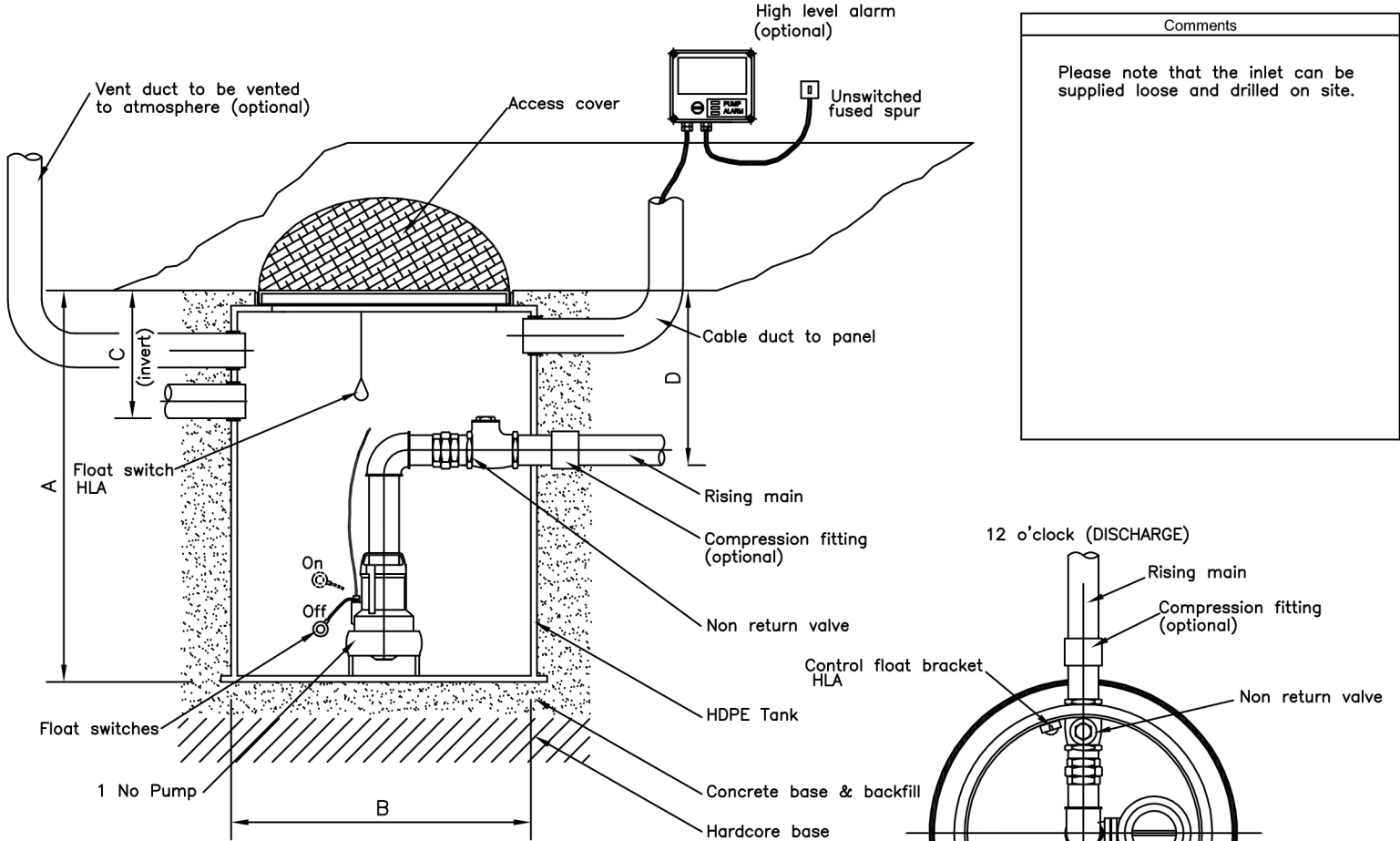
SIDE ELEVATION
